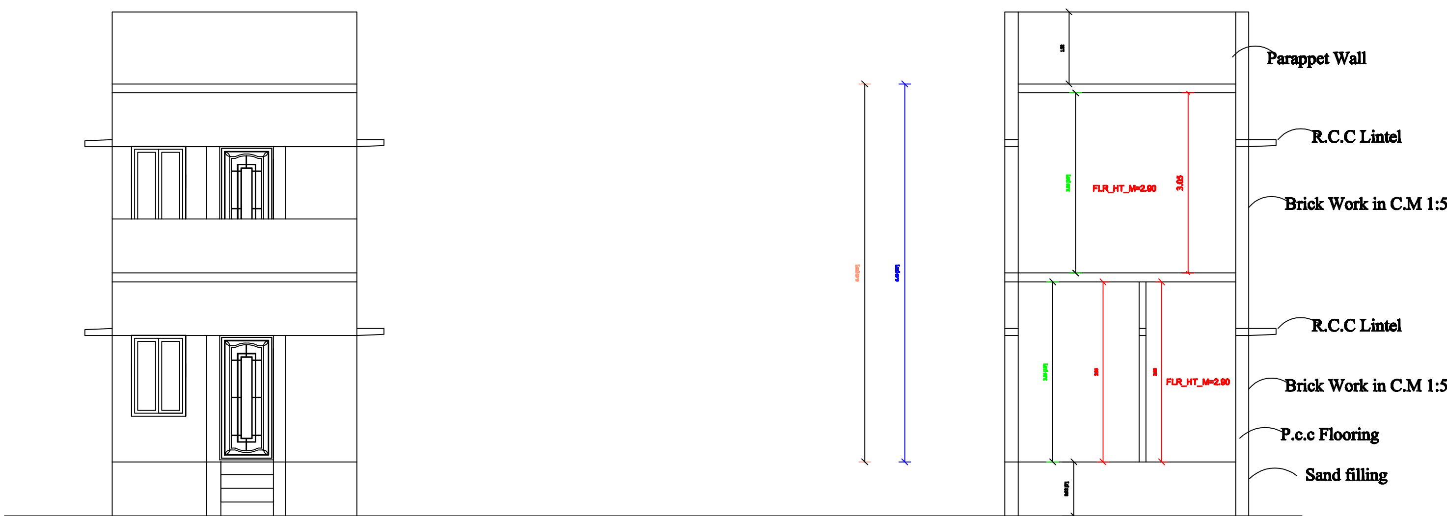
FRONT ELEVATION
