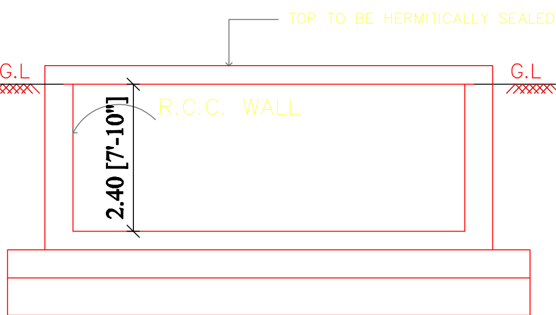
RWHS SECTION (SAMPLE)
