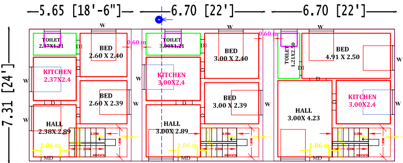
GROUND FLOOR PLAN (NORTH FACING)
