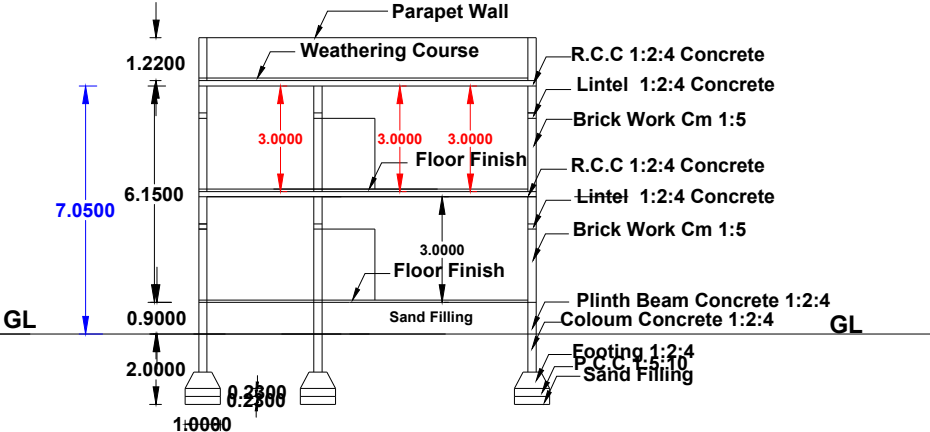
Section - XY
