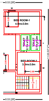
FLOOR PLAN
