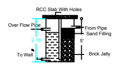
RWHS Tank Details
