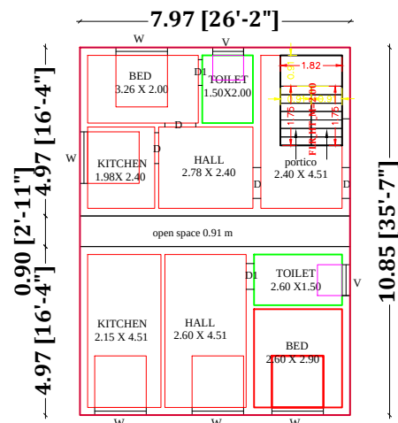
FIRST FLOOR PLAN EAST & NORTH FACING
