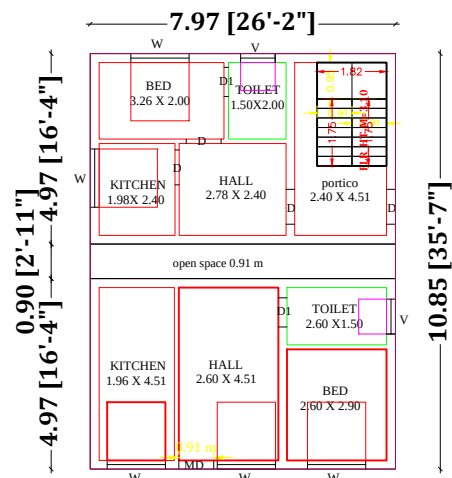
GROUND FLOOR PLAN EAST & NORTH FACING
