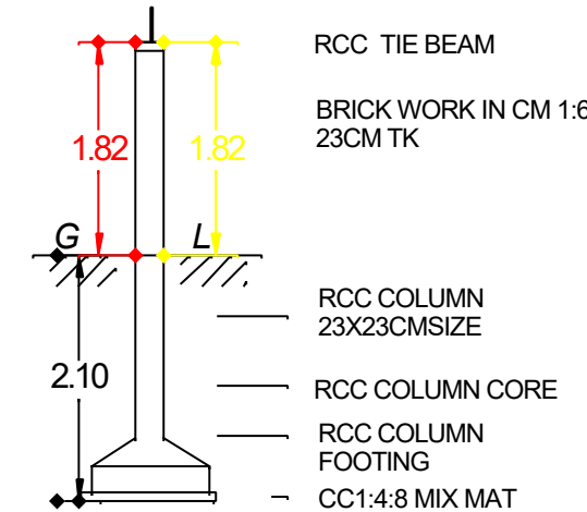
SECTION OF COMPOUND WALL DETAILS
