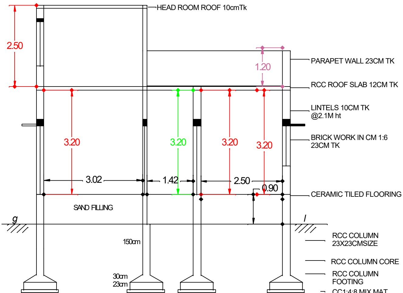
SECTIONAL ELEVATION ON X-X'AXIS
