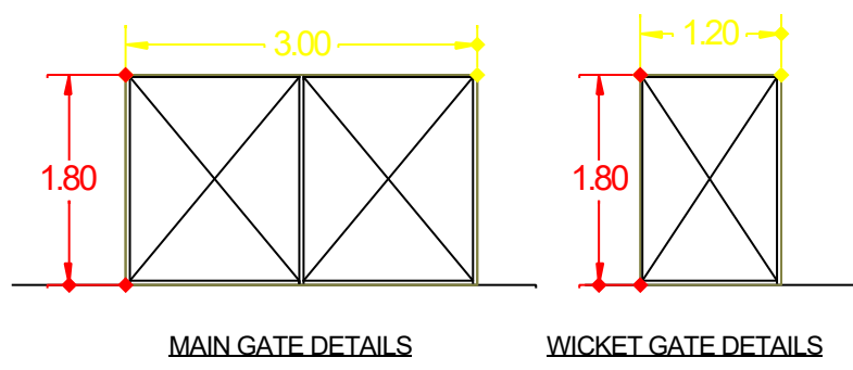
MAIN GATE DETAILS WICKET GATE DETAILS
