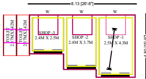
GROUND FLOOR COMMERCIAL PLAN
