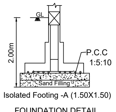
FOUNDATION DETAIL
