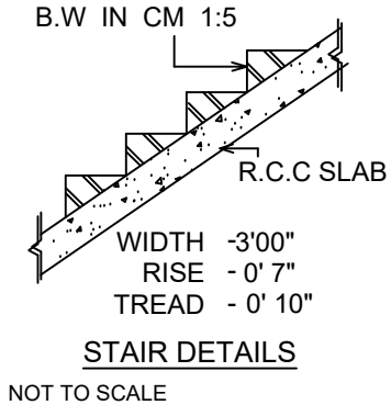
STAIR DETAILS
