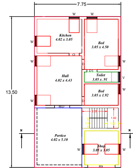
Proposed Ground Floor Plan North facing
