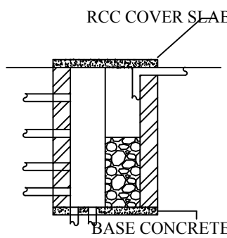
RAIN WATER COLLECTION PIT DETAILS NOT TO SCALE
