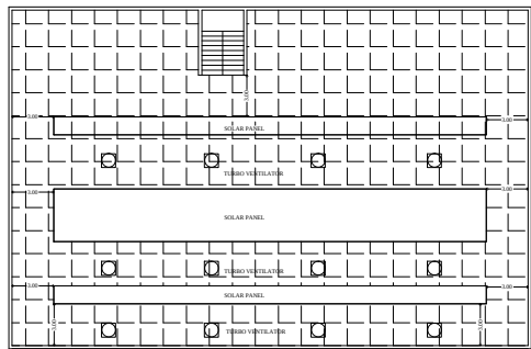
SHEET ROOF-TERRACE BLOCK - 2
