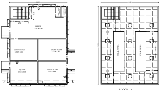
BLOCK - 1 GROUND FLOOR
