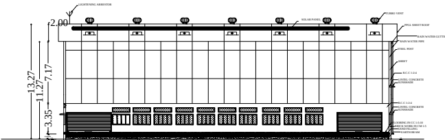
SECTION AA BLOCK - 2
