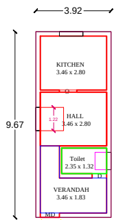
GROUND FLOOR PLAN EAST FACING
