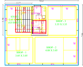
GROUND FLOOR PLAN (NORTH FACING)
