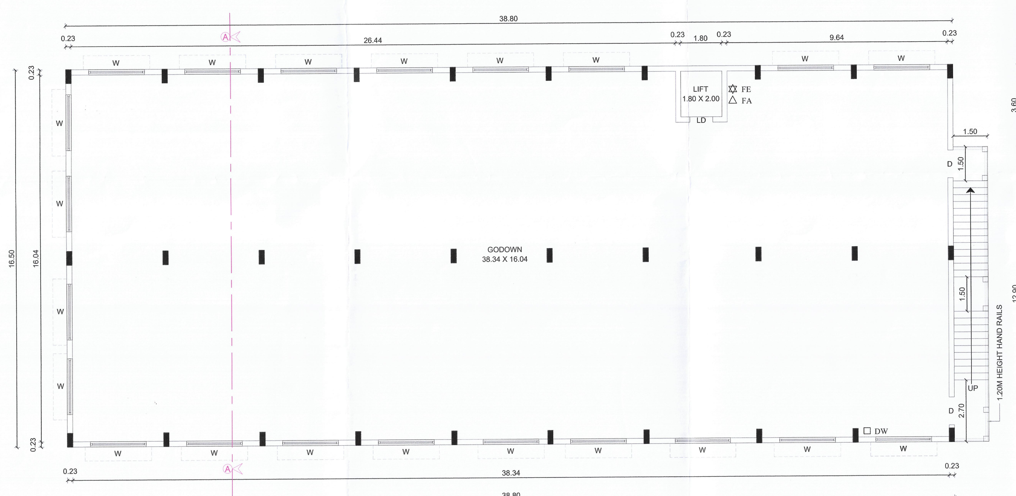
BLOCK-I FIRST FLOOR PLAN
