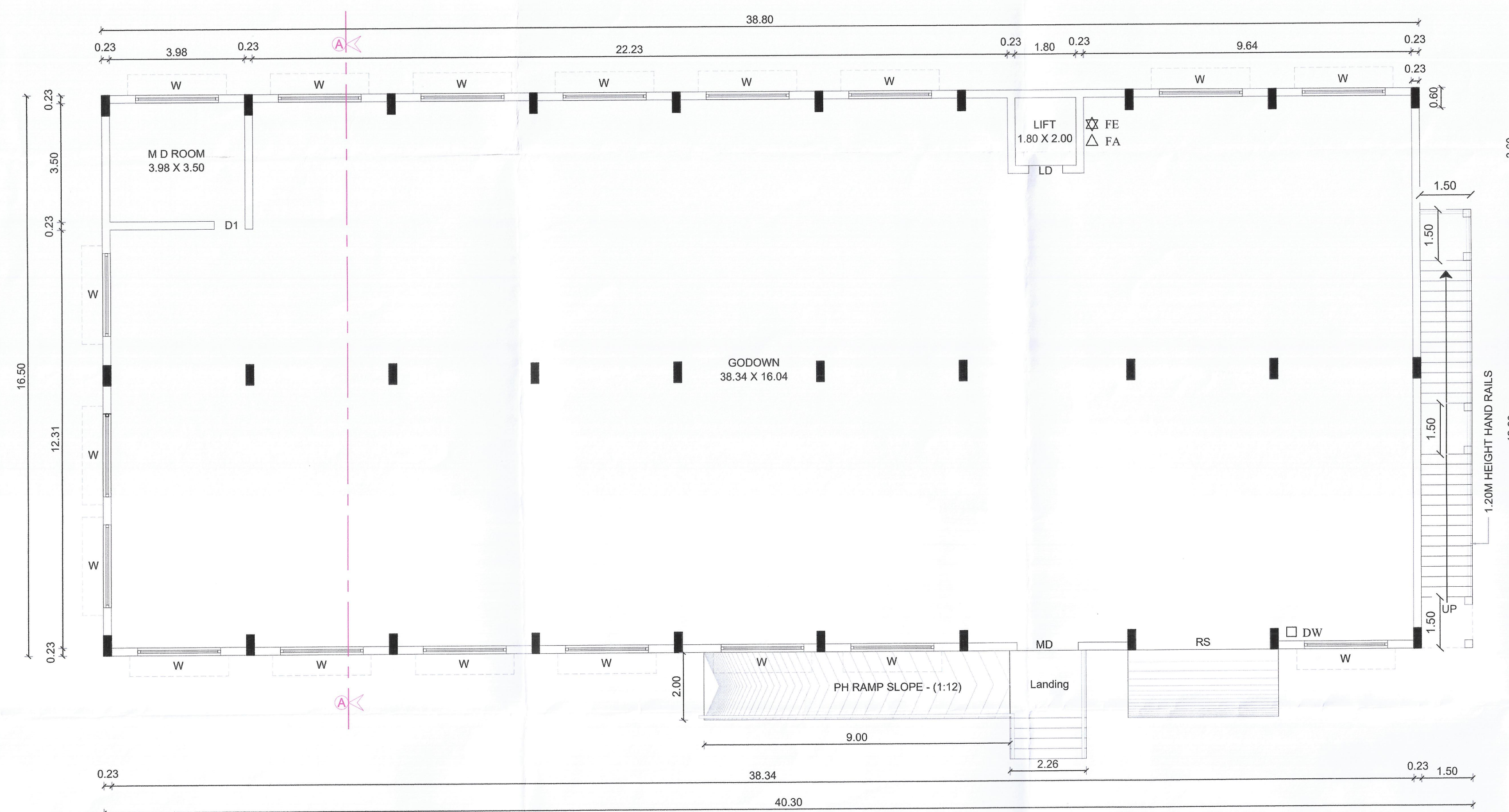
BLOCK-I GROUND FLOOR PLAN
