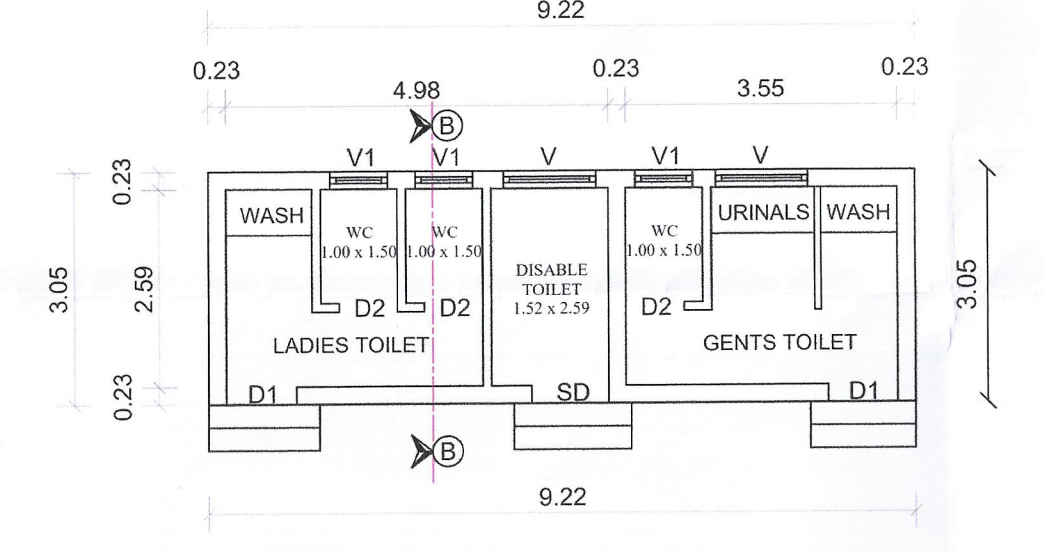
BLOCK-II GROUND FLOOR PLAN
