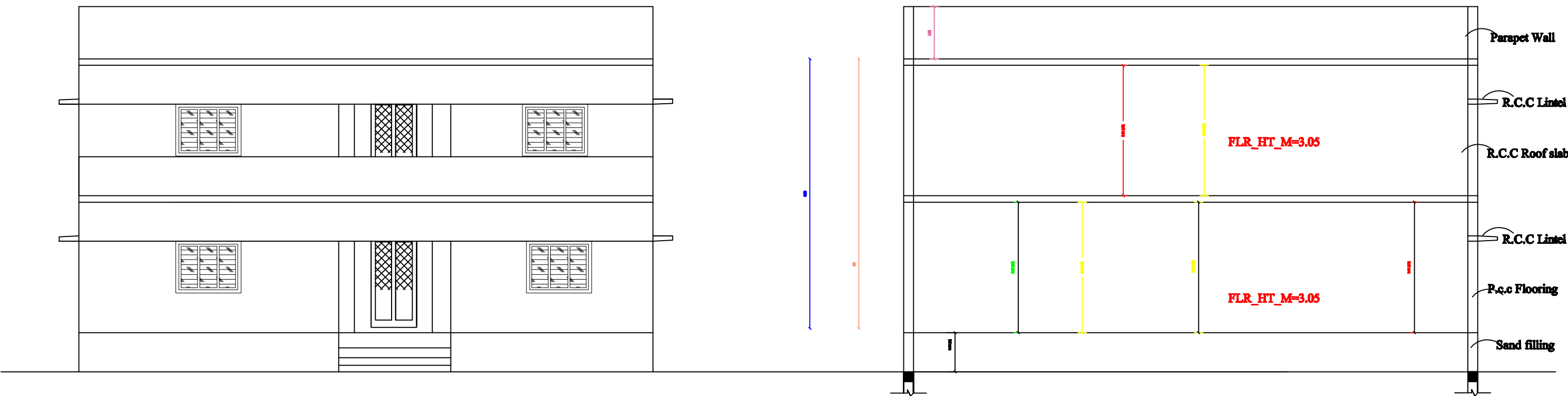
FRONT ELEVATION
