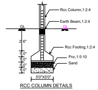
SCALE 1"=4'0"
