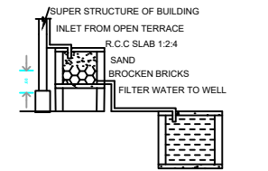
RAINWATER HARVESTING
