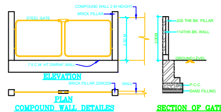
SECTION OF GATE
