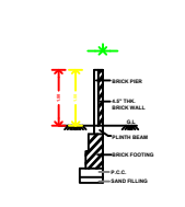
COMPOUND WALL DETAIL
