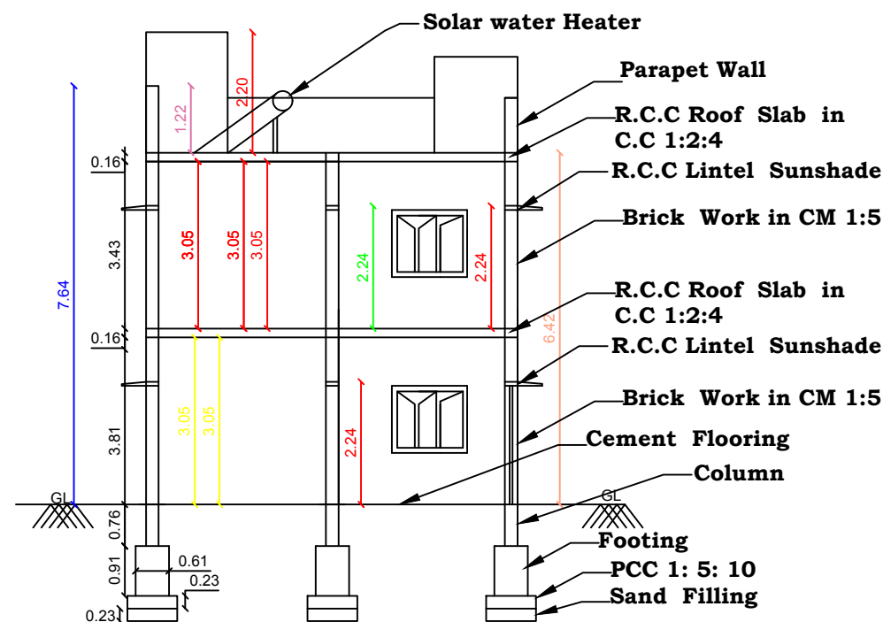
SECTION - BB
