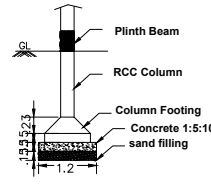
Column Footing Foundation Detail
