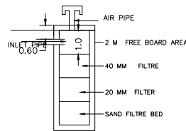
RWH_CAPACITY_L=3000LTRS
