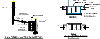
PLAN OF RAIN WATER HARVESTING
