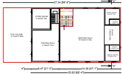
EXISTING GROUND FLOOR PLAN
