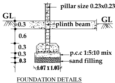
FOUNDATION DETAILS
