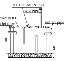
SEPTIC TANK SECTION
