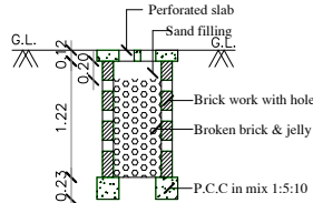
PERCOLATION PIT
