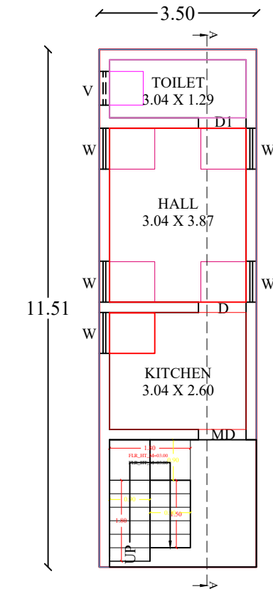
GROUND FLOOR PLAN (EAST FACING)
