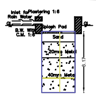
RAIN WATER PERCOLATION PIT
