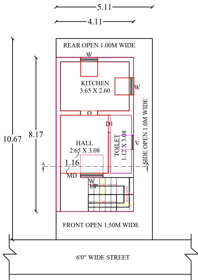
GROUND FLOOR PLAN (SOUTH FACING)
