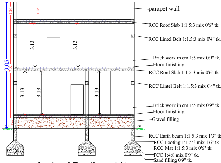
Sectional Details on AA'
