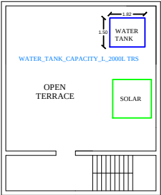
TERRACE PLAN
