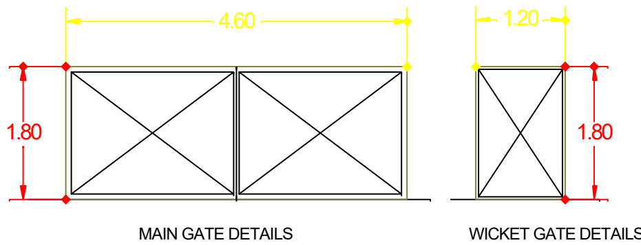
GATE DETAILS
