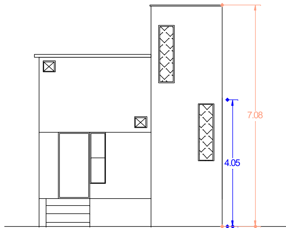
FRONT ELEVATION
