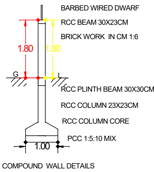
COMPOUND WALL DETAILS
