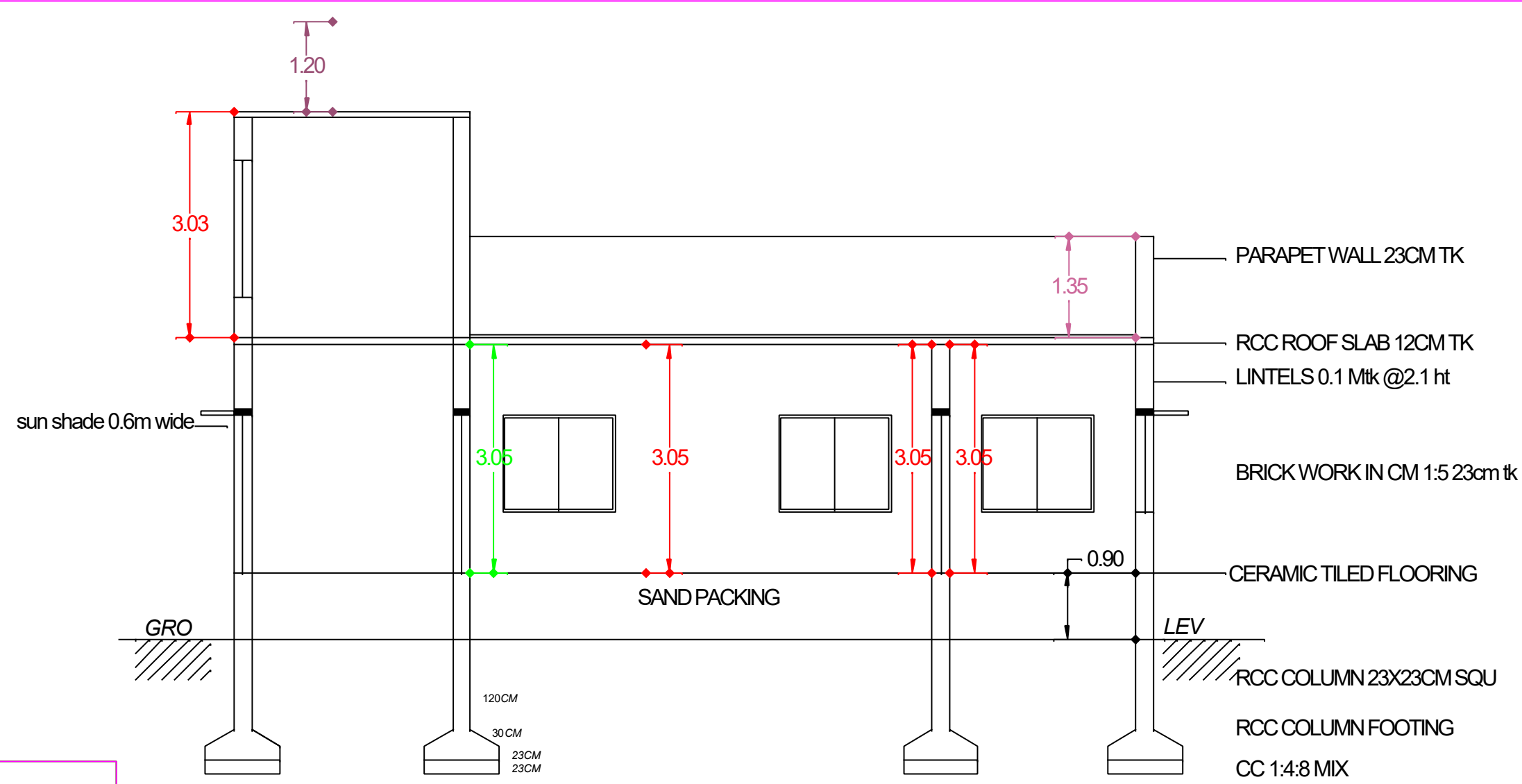
SECTION ON X X' AXIS
