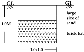
RAINWATER HARVESTING
