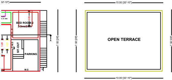
FLOOR PLAN
