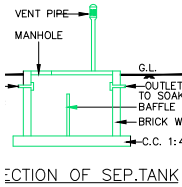
CROSS SECTION OF SEPT. TANK
