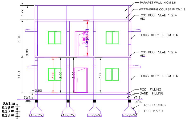
SECTION "A-B"
