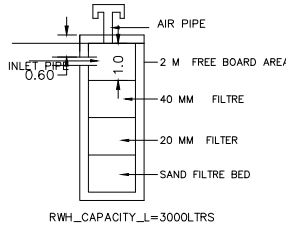
RWH_CAPACITY_L=3000LTRS
