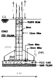
FOUNDATION DETAILS SCALE : 1:50.
