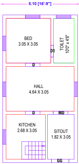
EX. GROUND FLOOR PLAN. [EAST FACING]
