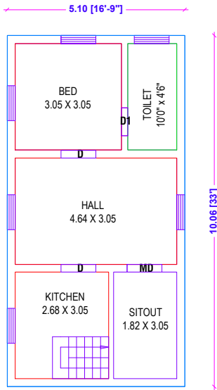
PRO. FIRST FLOOR PLAN. [EAST FACING]
