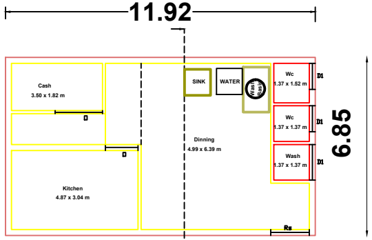
GROUND FLOOR PLAN BLOCK -2
