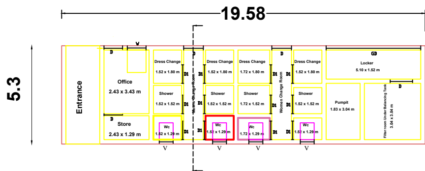
GROUND FLOOR PLAN BLOCK -1
