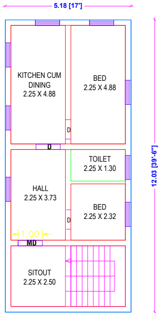
PRO. GROUND FLOOR PLAN. [NORTH FACING]
