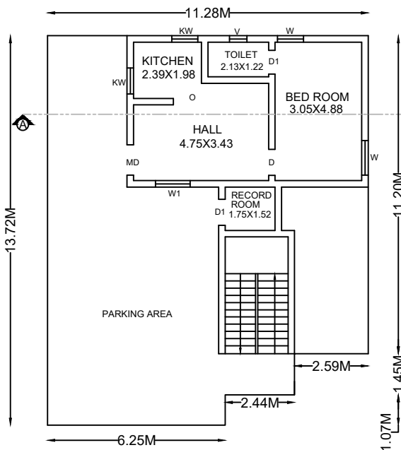
GROUND FLOOR PLAN (COMBINED FLOOR)
