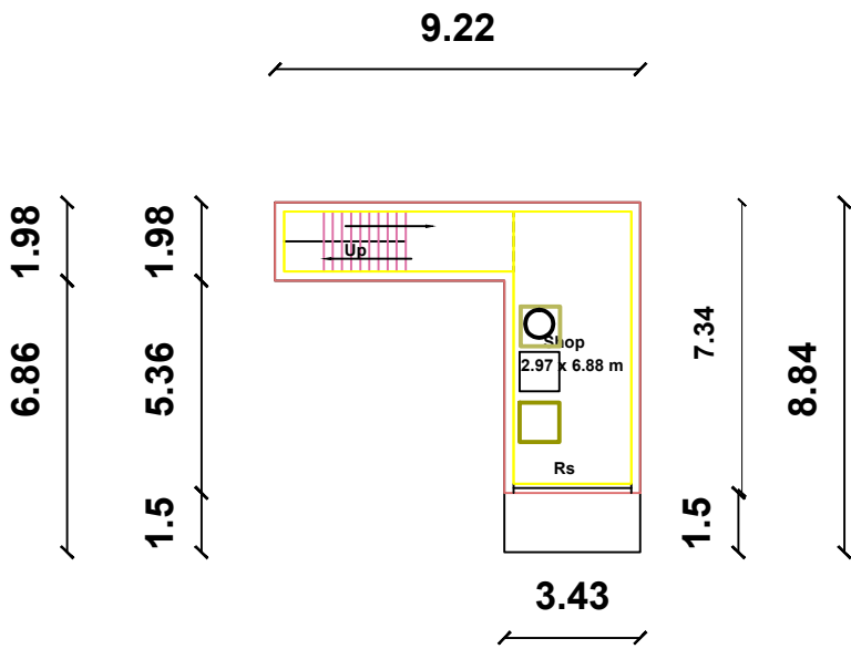
GROUND FLOOR PLAN ( SHOP )
