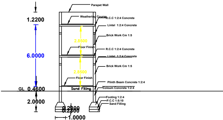
Section Section - AA
