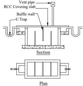
Waste Water Recycle Unit Not To Scale
