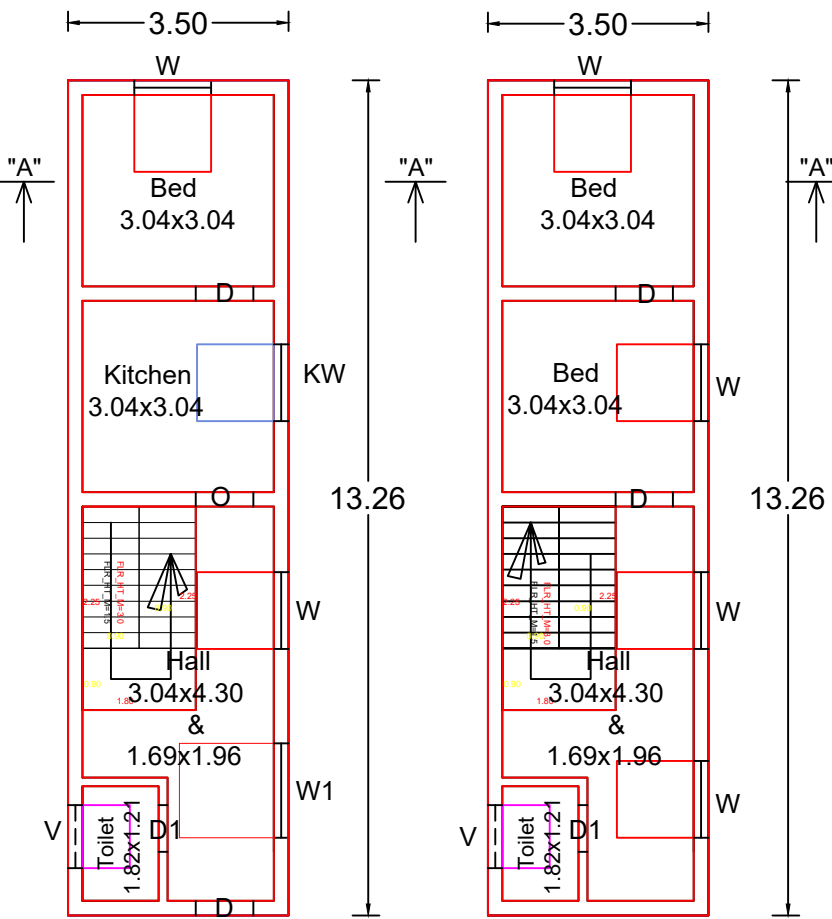
PLAN - G.F.
