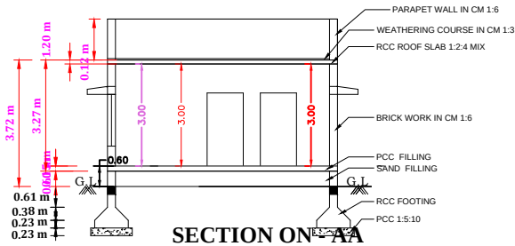
SECTION ON-AA
