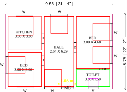
GROUND FLOOR PLAN NORTH FACING
