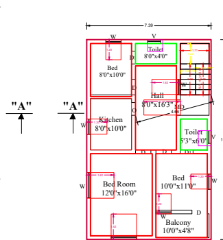
PROPOSED FIRST FLOOR PLAN
