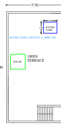
TERRACE PLAN
