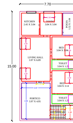
GROUND FLOOR PLAN NORTH FACING
