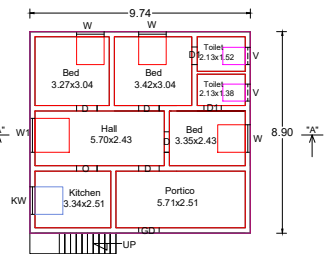
PLAN - G.F ( FACING: EAST)
