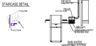
STAIRCASE DETAIL
