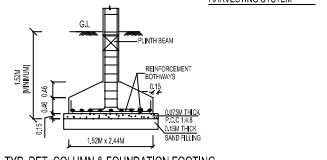
TYP. DET. COLUMN & FOUNDATION FOOTING
