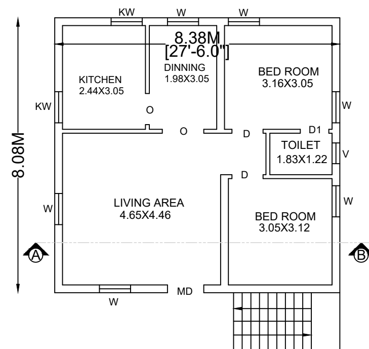
GROUND FLOOR PLAN (NORTH FACING)
