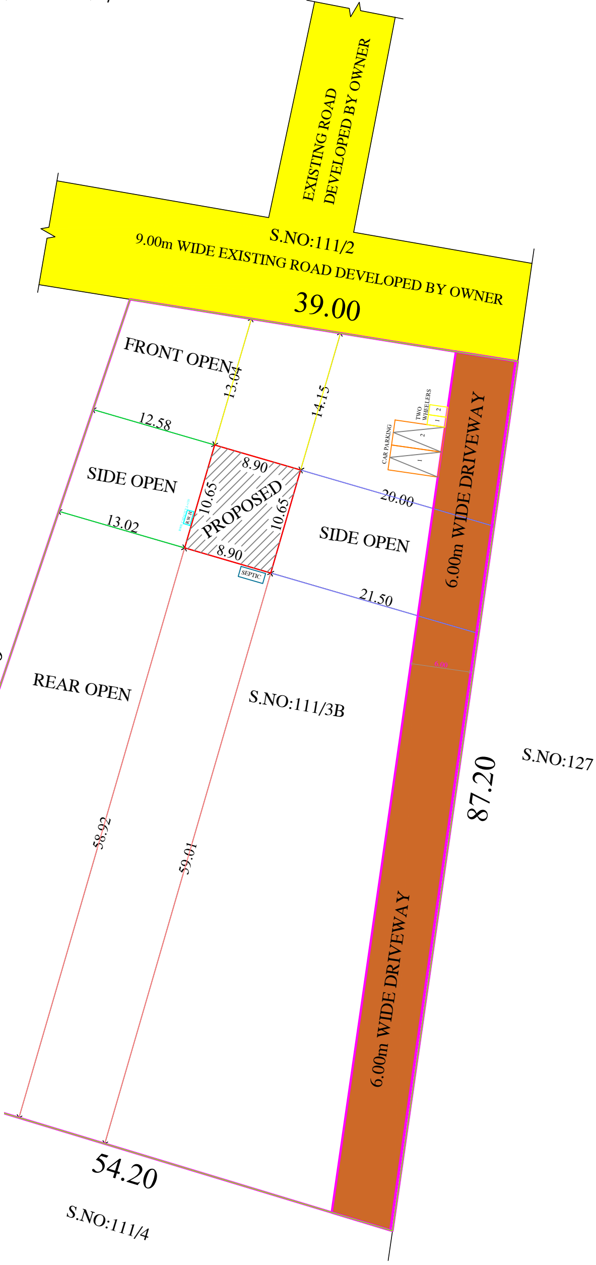
SITE PLAN
