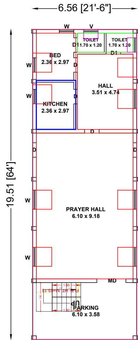
GROUND FLOOR PLAN (EAST FACING)
