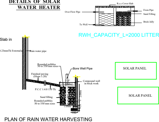
PLAN OF RAIN WATER HARVESTING
