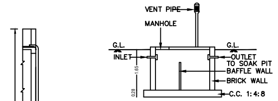
SECTION OF SEP.TANK
