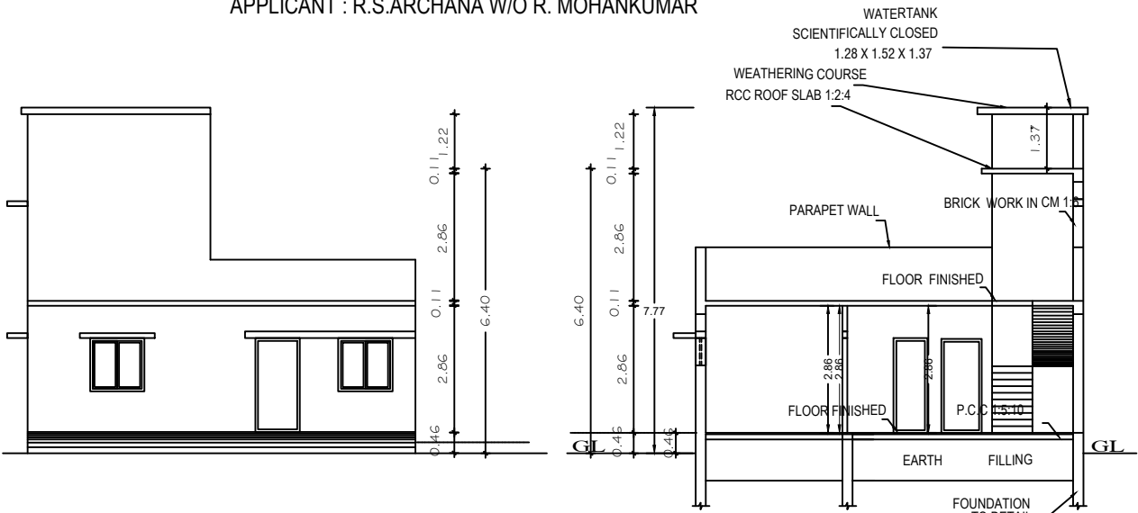
FRONT ELEVATION.
