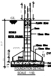
FOUNDATION DETAILS
