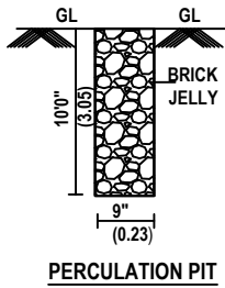
PERCOLATION PIT
