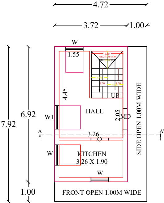
GROUND FLOOR PLAN EAST FACING)
