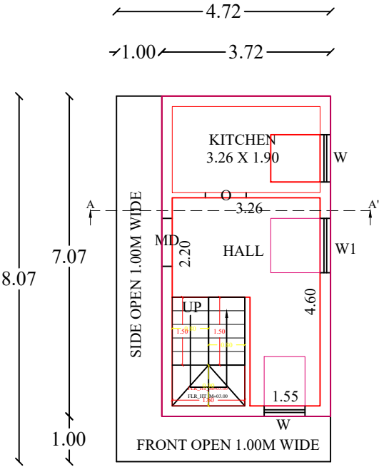
GROUND FLOOR PLAN WEST FACING)
