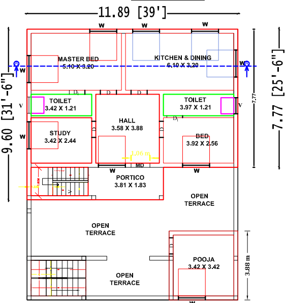
FIRST FLOOR PLAN (WEST FACING) PROPOSED
